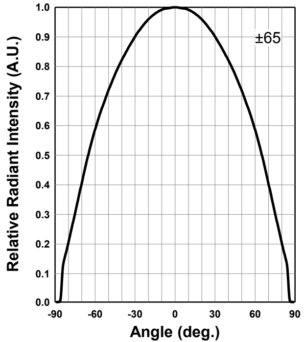
Radiation Characteristics
