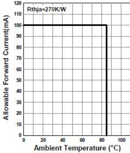
Allowable Forward Current - Ambient Temperature
