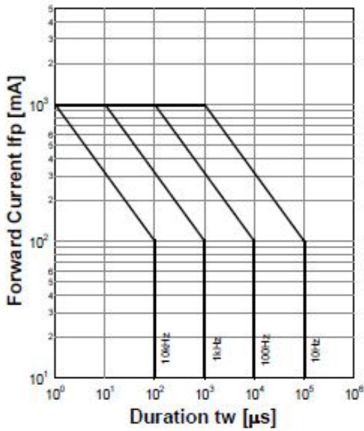
Forward Current - Pulse Duration
