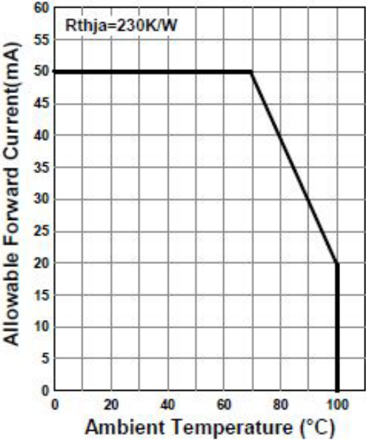
Allowable Forward Current - Ambient Temperature
