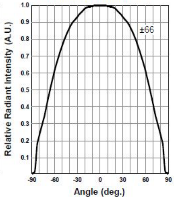
Radiation Characteristics
