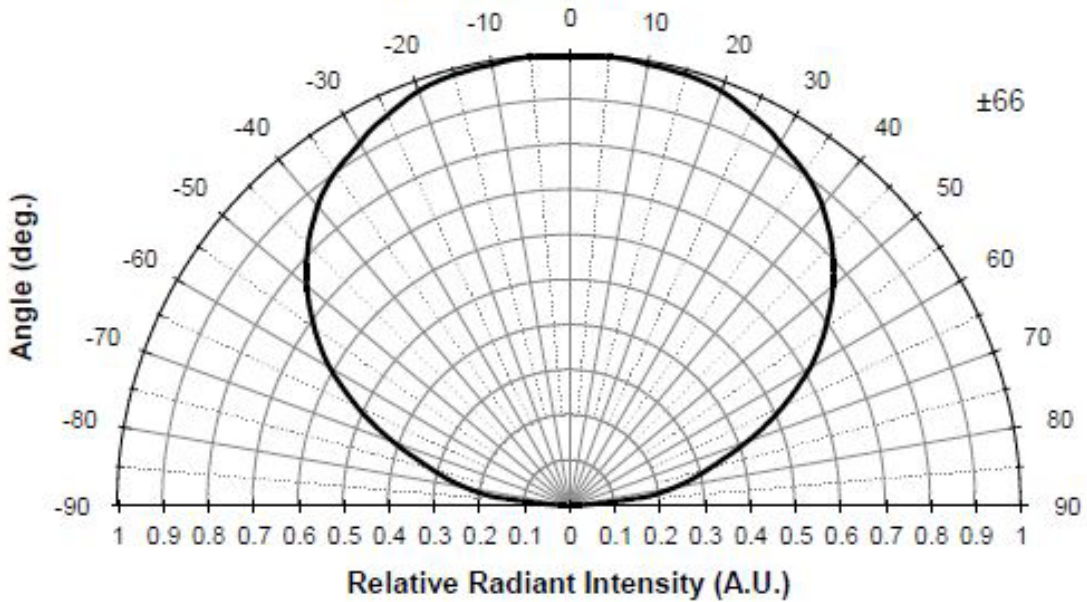
Radiation Characteristics
