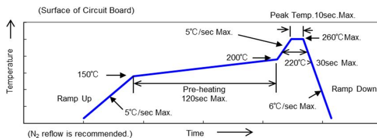
Reflow soldering profile
