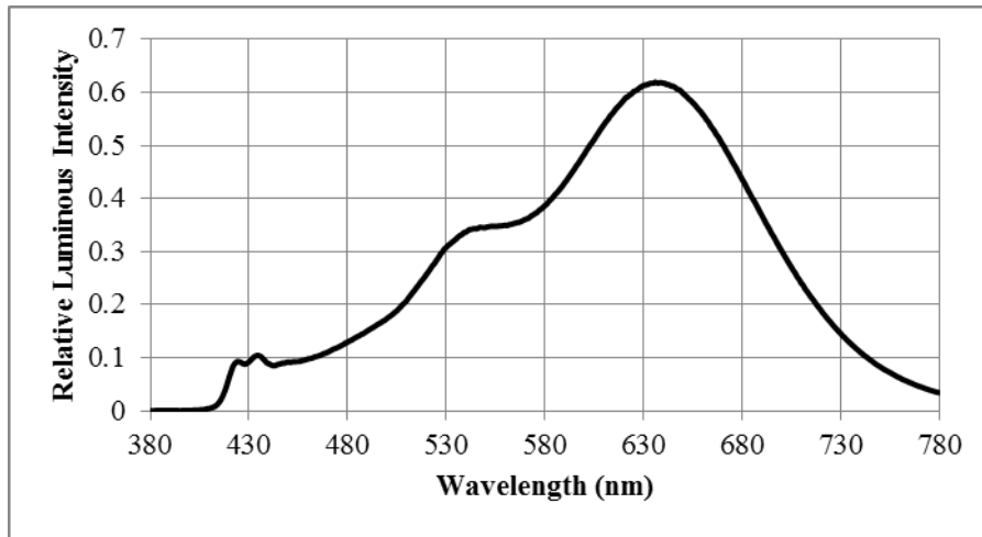
Spectrum (Ta=25°C, I f =65mA)
