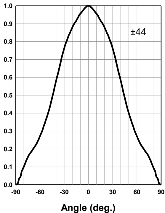
Radiation Characteristics
