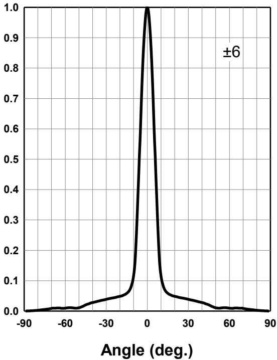
Radiation Characteristics
