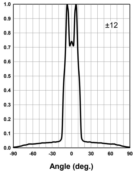
Radiation Characteristics
