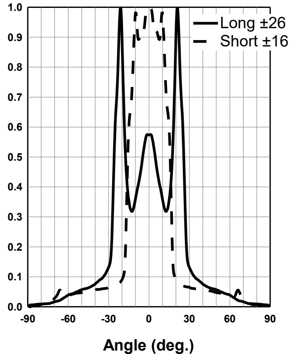
Radiation Characteristics
